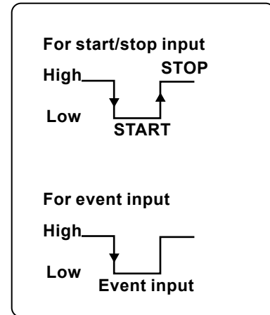
Input signal waveform
