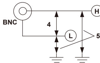
Combined with the (701901 + 701954) or direct input (cable that does not comply with the safety standards)
