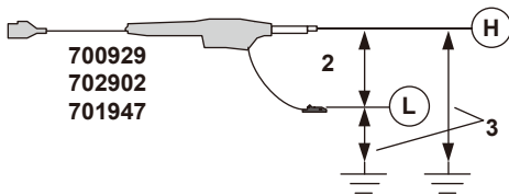
Direct input (cable that does not comply with the safety standards)
