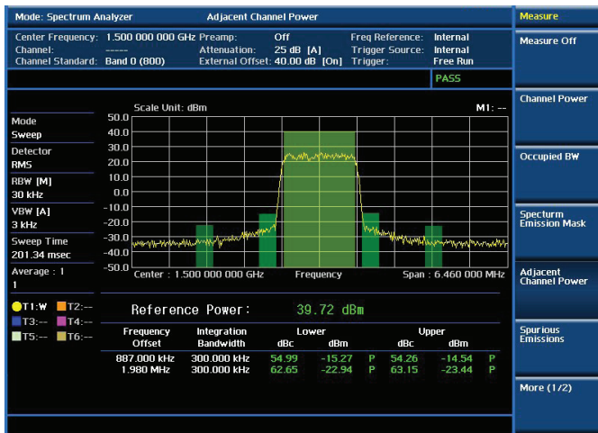
RF test — Adjacent Channel Power
