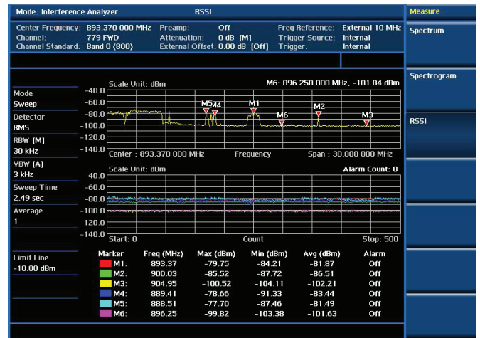
Interference analysis test — RSSI
